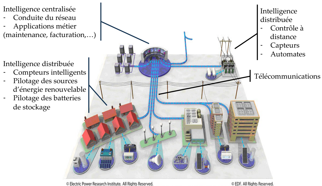
FIGURE 1.2 – Architecture des Smart Grids [2006-1]
